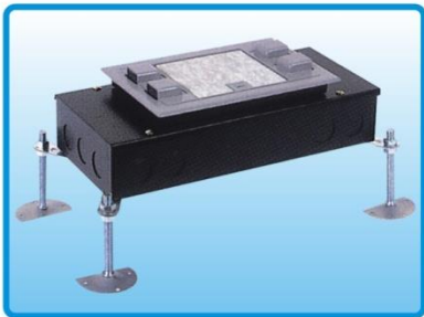
KM-02 AL(알루미늄)-P9
